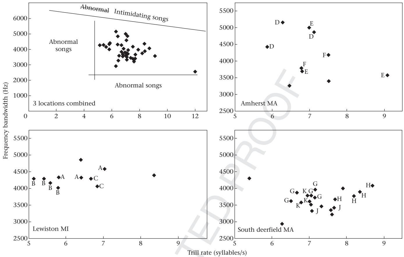
Figure 6. Scatterplots of trill rate and frequency bandwidth for swamp sparrows from three locations, revealing that scatter is largely due to song types (letters A–K; song types deemed unique to an individual are not labelled), leaving little if any information available about the quality of individual singers. In the upper left, data for all three locations are combined, and the axes meet at the origin (0,0); the graphs for the three separate locations are drawn to a different scale, expanded to better show the variation within locations (note that the outlying data point at 12 syllables/s is omitted from the lower-right graph; excluding it has no bearing on the conclusions to be drawn from this figure). The upper-bound line in the upper left subfigure is from Ballentine et al. (2004); the bounds below and to the left of the data points are placed arbitrarily. In the three subplots, letters label different renditions of a given song type from different males; because of local dialects, song types were not shared across locations.
