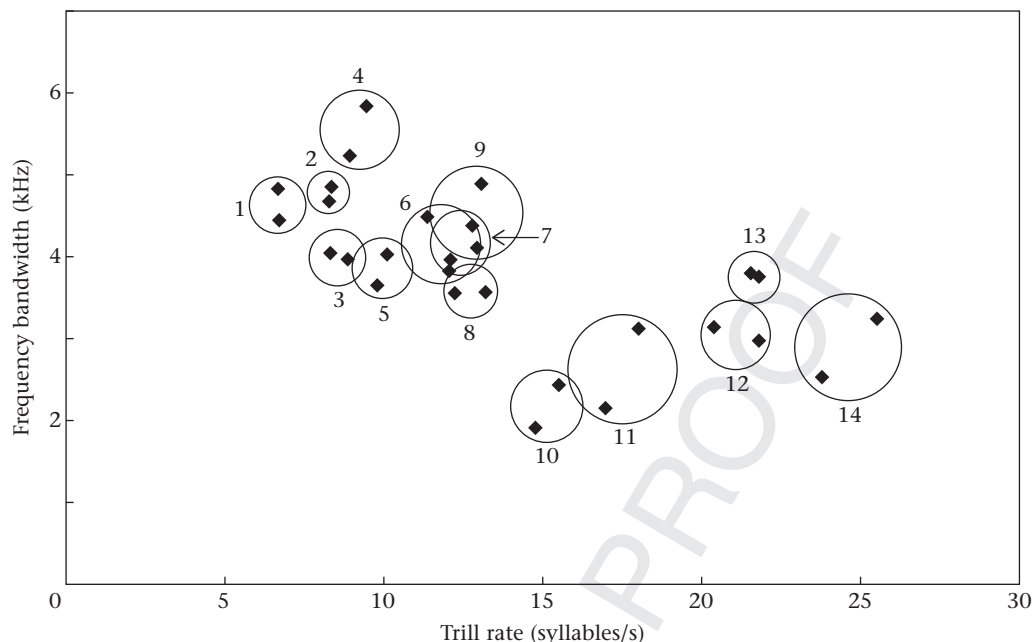
Figure 5. All aspects of a male chipping sparrow's song, including the trill rate and frequency bandwidth, are determined largely by the song that he imitates from an adult male, so that song types dictate the scatter in the plot, not relative male quality. Plotted data are from Fig. 2, and each of the 14 circles encompasses the songs of two neighbouring males.
