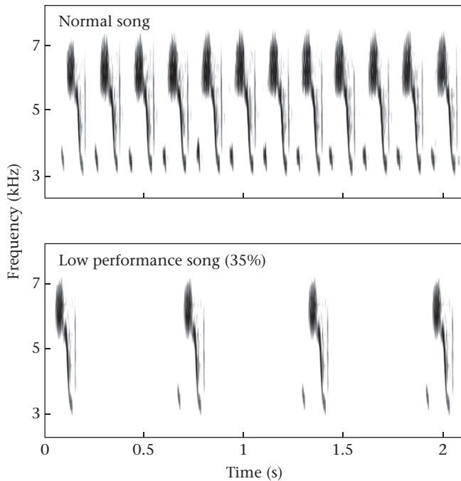
Figure 10. To produce playback stimuli, Moseley et al. (2013) altered a normal song (top) by adding or deleting silent spaces between the song elements. In this illustration (bottom), silent intervals are increased 8.3 times, producing a highly abnormal song with four syllables delivered at 35% the rate of normal.
