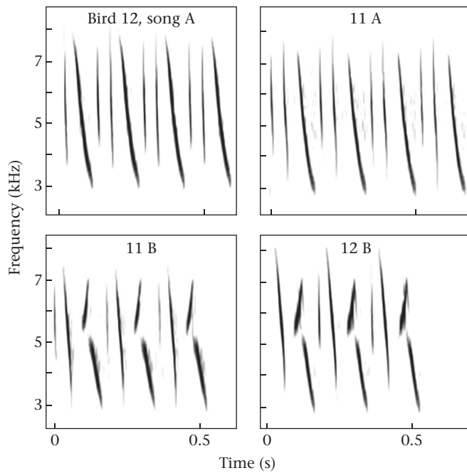
Figure 7. Swamp sparrow males within a marsh learn their songs from one another and, as a result, many songs are shared among birds in a population. From Lewiston, Michigan, U.S.A., examples are illustrated for two different song types (A and B). Songs of higher performance (lower deviation from the upper bound, as shown in upper left of Fig. 6) are in the second column. Birds 11 and 12 were immediate neighbours; bird 11 had the 'better' A song, bird 12 had the 'better' B song.
