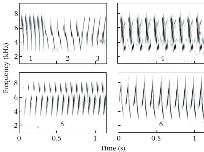
Figure 3. During the dawn chorus, chipping sparrow males can gather in lek-like, competitive singing arenas well away from their daytime territories. In this example, during the dawn chorus, four males (1–4) gathered in a lek-like arena on a paved road, displaying with brief songs in the dark, sight unseen (the half-second song fragment of bird 2 is a typical dawn song); individuality in their songs allowed each to be identified. After the dawn singers had dispersed to their daytime territories, two other males (5, 6), who presumably were elsewhere during the dawn chorus, sang at this location on their daytime territories; their songs were far longer, abbreviated to 1 s here only for illustration.
