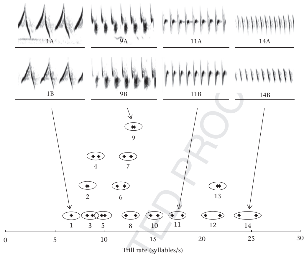
Figure 2. A few dozen different song types can occur within a chipping sparrow population (only four illustrated here: 1, 9, 11, 14), but neighbouring males (A and B) often have nearly identical songs, the result of a young male copying the song of a nearby adult singer (Liu & Kroodsmas, 1999, 2006); all features of a male's song, including his trill rate as illustrated here (14 examples), are determined by that adult tutor. In the lower graph, each oval encircles the two data points (pairs 1 and 2 are identical) for trill rates from two neighbouring males with the same song types (data are distributed vertically for easier visibility). Each data point is the median of three measurements for a given male.
