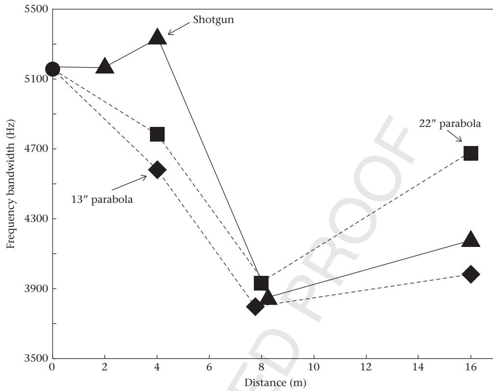
Figure 9. The frequency bandwidth of a chipping sparrow song, as measured in performance studies, varies not only with (1) the microphone used but also with (2) the distance to the singing subject. A chipping sparrow song was broadcast from a JBL Pro III speaker under calm, quiet conditions (midnight) and recorded at 2, 4, 8 and 16 m; the speaker was perched 1 m above the ground, with a direct line of sight beside several small bushes over the 16 m distance. The bandwidth value reported for 0 m was measured directly from the WAV file that was later broadcast through the speaker. Each plotted value is the median of three measurements for successive broadcasts of the same song. Microphones tested: Sennheiser ME66 shotgun, 13-inch (33 cm) Sony PBR330 parabola, 22-inch (56 cm) Telinga parabola (both parabolas with Sennheiser MKH20 microphone). Furthermore, bandwidth also varies with a third variable, song type, as four additional song types revealed strikingly different transmission patterns among them (for the ME66 shotgun, bandwidths for all five song types ranged from 83 to 104% of the original WAV file at 4 m, 74 to 100% at 8 m and 72 to 107% at 16 m).
