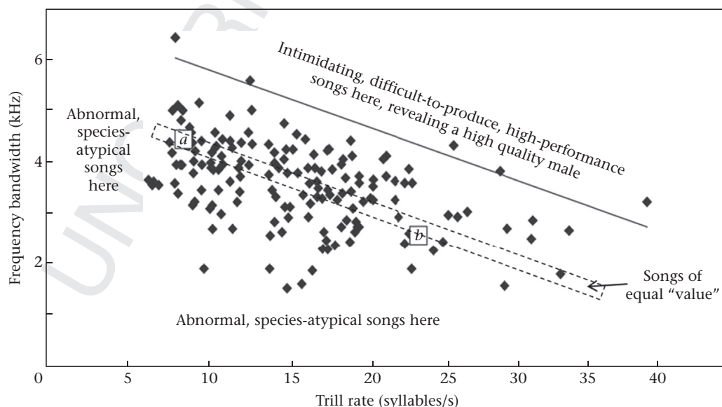
Figure 4. Reprinted with permission from Figure 1 in Goodwin and Podos (2014). 'Chipping sparrow songs show evidence of a vocal constraint ... Biplot of trill rate and frequency bandwidth ( N = 160 males) reveals a performance trade-off in vocal production'. Letters 'a' and 'b' refer to a portion of the original figure not illustrated here. Songs that plot within the dashed rectangle have similar deviations from the upper bound and would therefore be considered equally good, or proficient, in other performance studies. Data are replotted on expanded axes to show the open space below and to the left of the data points.
