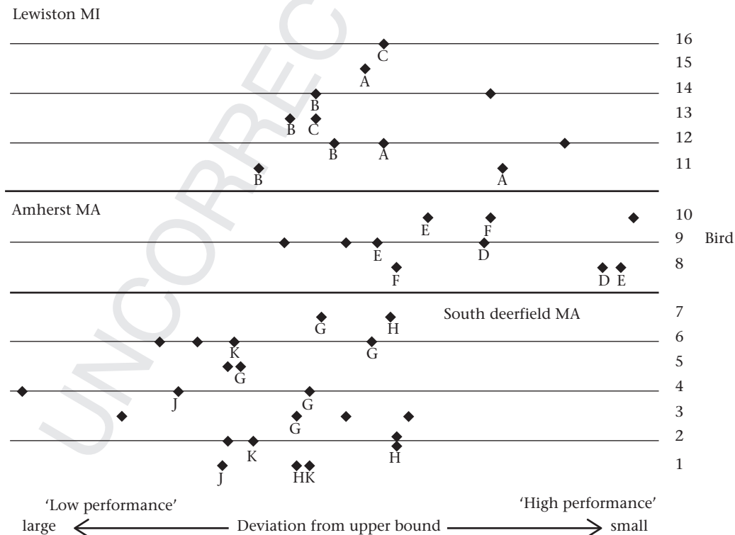
Figure 8. Song performance measures can provide no reliable information about inherent male quality in swamp sparrows. Data plotted here have been extracted from Fig. 6 by measuring the shortest distance to the upper bound for each song (all measures are relative, depending on a number of factors, so no absolute scale is provided for performance). Performance measures for different males are broadly overlapping, such that a male might have the highest performance on one of his song types but the lowest on another (e.g. compare bird 3 from South Deerfield with birds 1, 2, 5, 6 and 7; song types are lettered as in Fig. 6). Note that Amherst swamp sparrows significantly 'outperform' the South Deerfield birds only 20 km distant (the two populations were recorded within a few days of each other during late June 2015; I can think of no methodological issues that would have produced such results).
