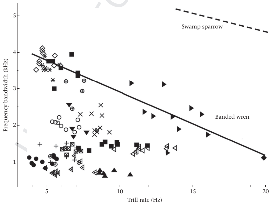
Figure 11. Reprinted with permission from Figure 1 in Illes et al. (2006). 'Graph of trill rate versus frequency bandwidth for 695 trills recorded from 13 individuals and including 16 trill types. Each symbol type represents a different trill type. The banded wren upper-bound limit is shown with a solid line and the swamp sparrow limit (Ballentine et al. 2004) with a dashed line.' Note that, as is usual for these graphs, the axes do not meet at the origin (0,0), and thus do not reveal the 'atypical space' below and to the left of the data.
