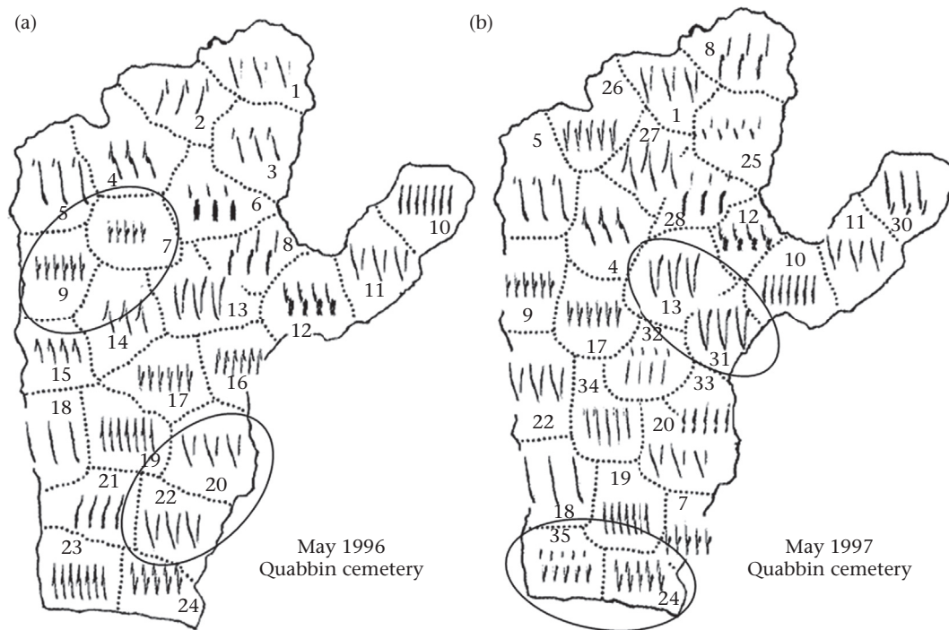
Figure 1. Reprinted with permission from Figure 2 in Liu and Kroodsma (2006). ‘Yearling’ Chipping Sparrows imitate songs of an immediate neighbour, but the instability of territories results in only short-term song sharing among neighbours. (a) In May of 1996, 24 territorial males (numbered 1–24) were found in the Quabbin Cemetery, and a portion of each male’s song type (0.35 sec) is illustrated. Males 7 and 9 share similar song types, as do males 20 and 22. (b) In May of 1997, 26 territorial males were found in the cemetery, 16 returning adults (at least two years old) from the previous year and 10 birds breeding there for the first time. Males 7 and 9 both returned but are no longer neighbours, and male 22 did not return. Male 35 did not learn the song of his father (male 5) or his father’s close neighbour in 1996 or 1997, but instead appeared to learn from his immediate neighbour in 1997 (male 24). Male 31 also appeared to acquire his song from an immediate neighbour (male 13) in 1997, not from his father (male 10). Both 1997 yearlings (31 and 35) hatched late in the 1996 breeding season, and each most likely acquired his song during 1997, as a yearling’.
